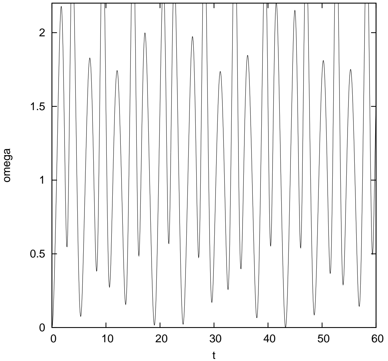
Orbiting Dumbbell Problem Circular Orbit -- Tolerance=10(-12)
