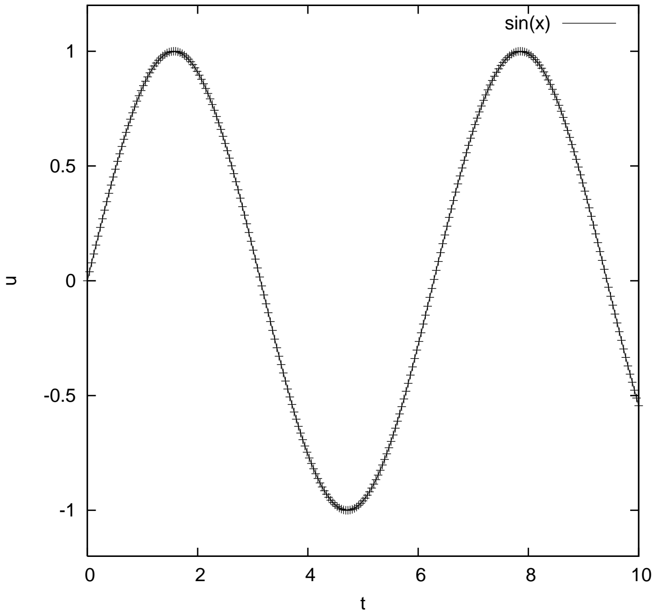
LSODA integration of u''(t) = -u(t)
