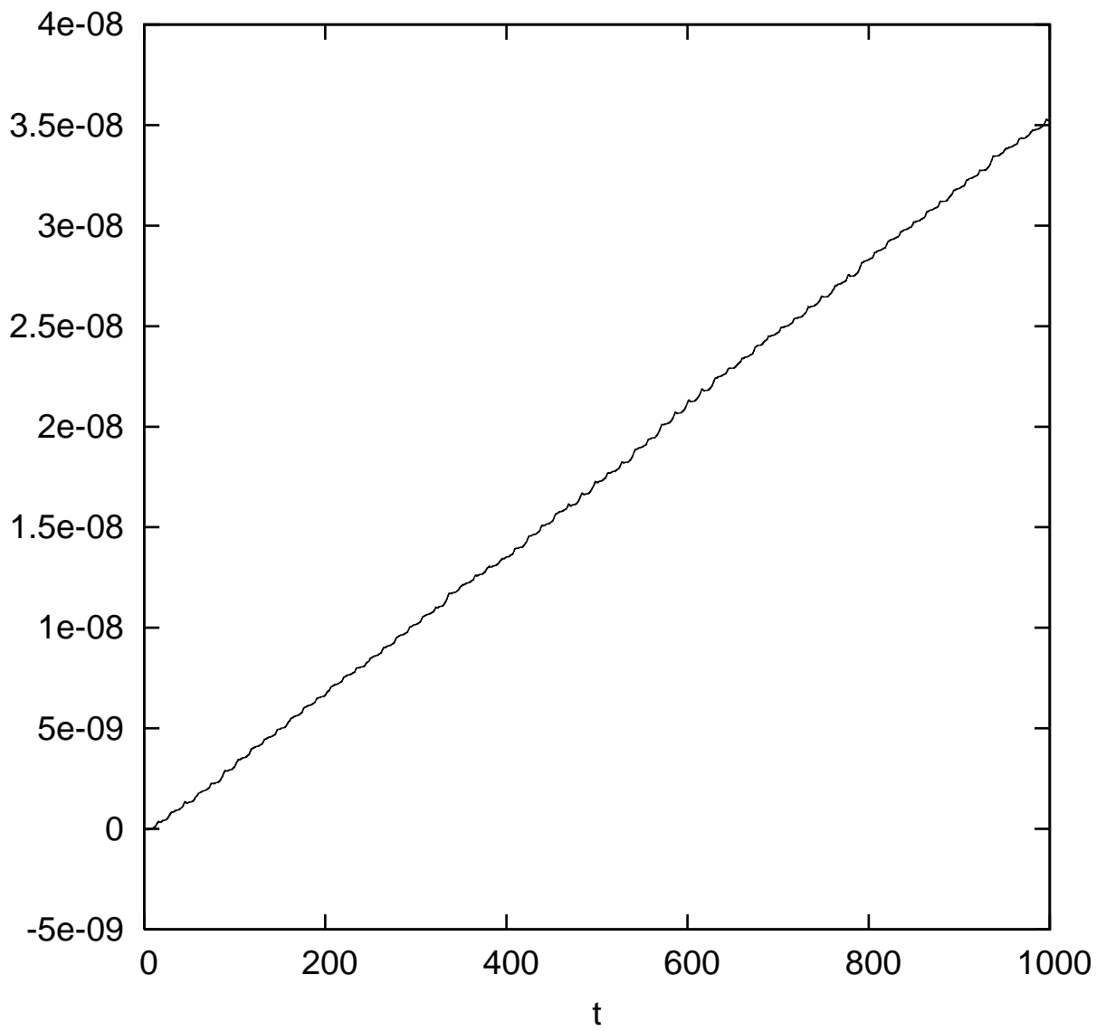
Orbiting Dumbbell Problem Elliptical Orbit -- Deviation in Total Energy -- Tolerance=10(-12)
