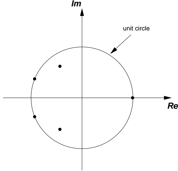
Figure 2: Schematic illustration of location in complex plane of eigenvalues of update matrix \mathbf{G} . In this case, all eigenvalues (dots) lie on or within the unit circle, indicating that the corresponding finite difference scheme is stable.
