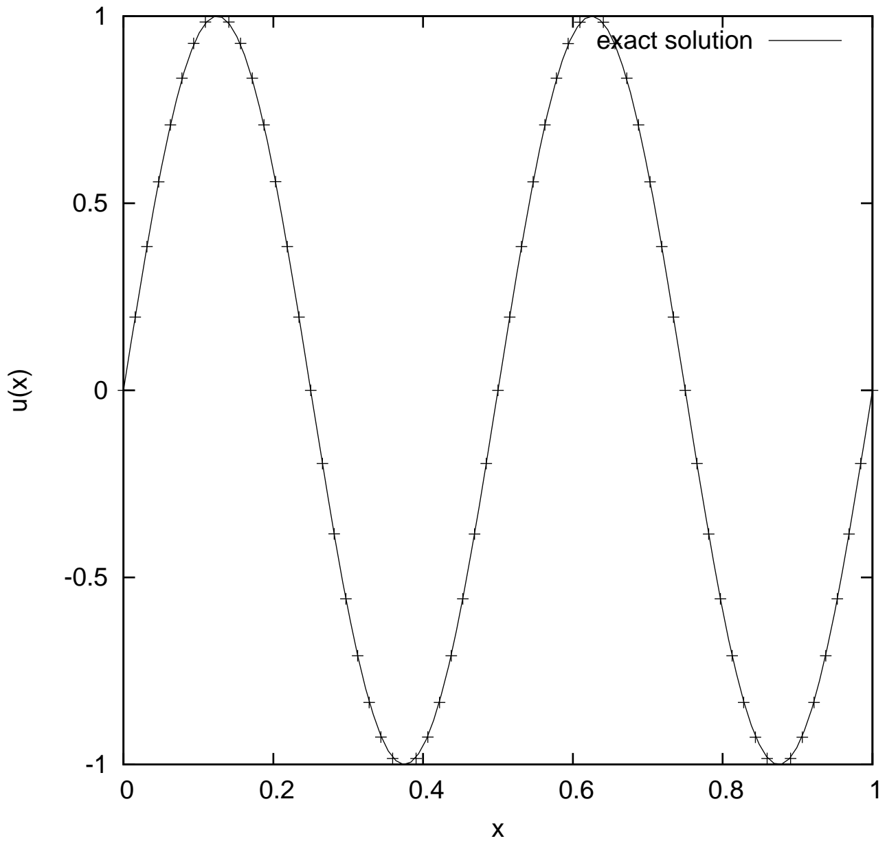
Solution of Nonlinear BVP guess_factor = 1.0
