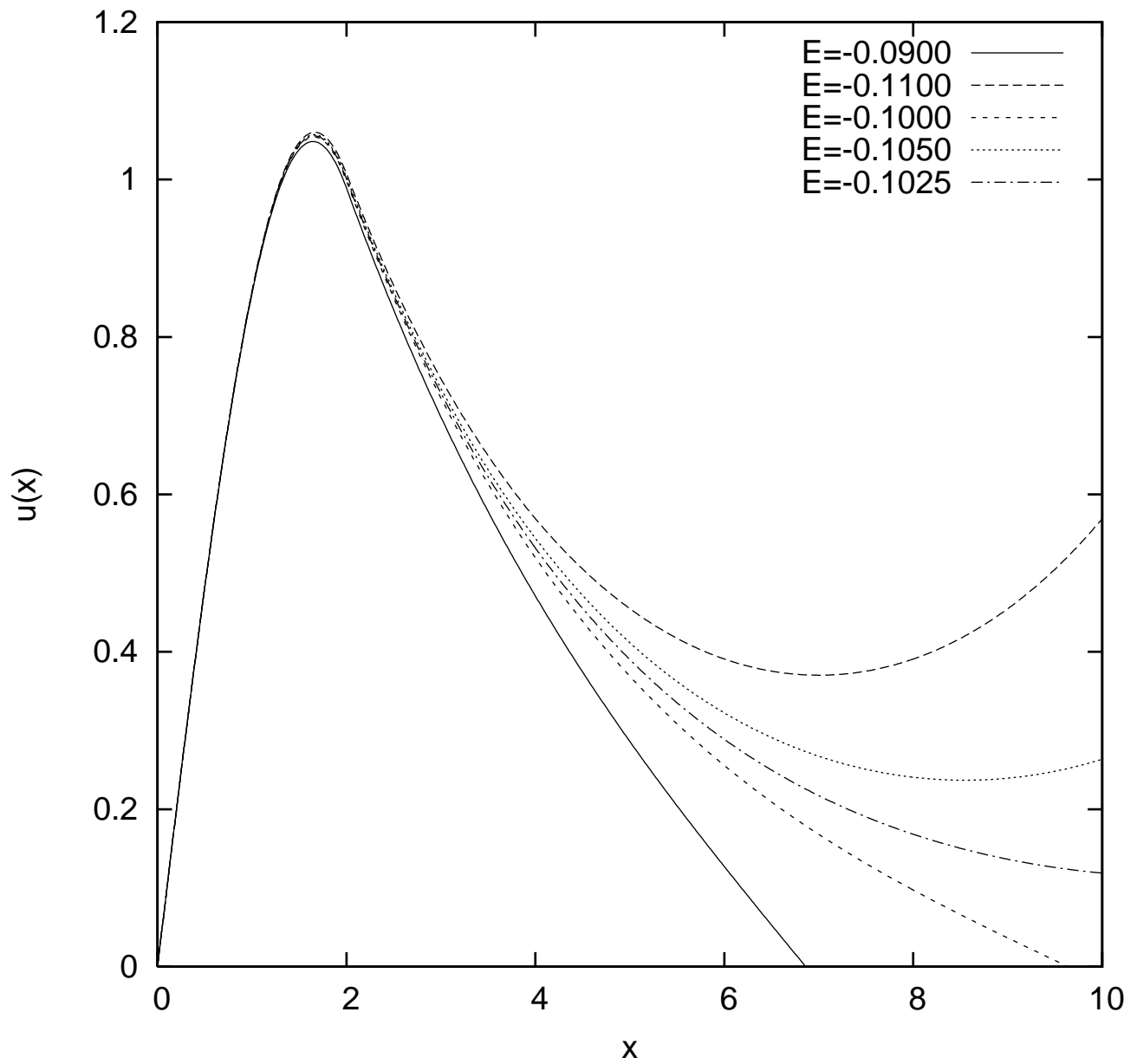
Toy Model Deuteron Wave Functions Unit depth square-well potential with range x_0=2.0 Illustration of bisection solution for eigenvalue (detail)
