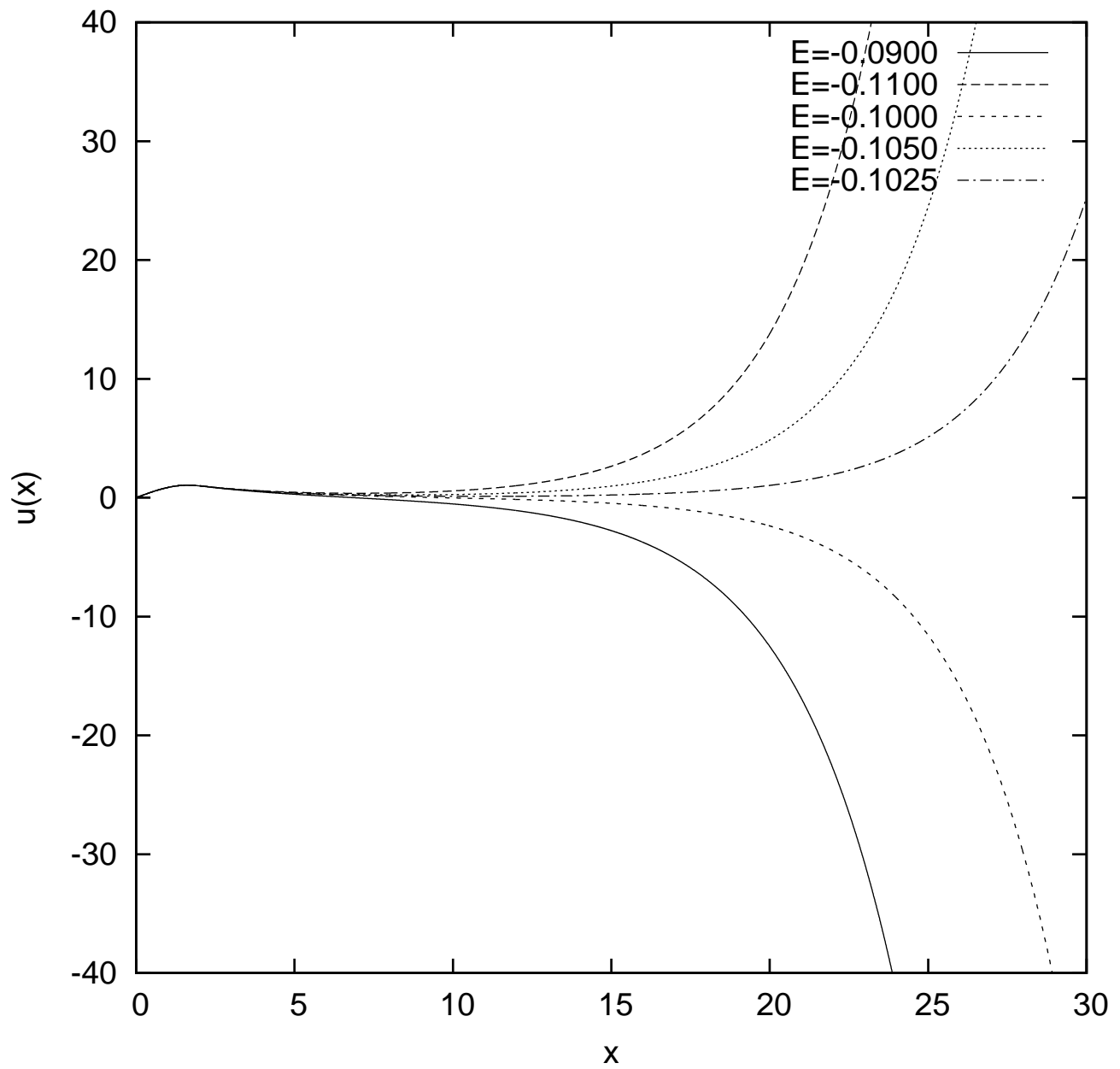
Toy Model Deuteron Wave Functions Unit depth square-well potential with range x_0=2.0 Illustration of bisection solution for eigenvalue
