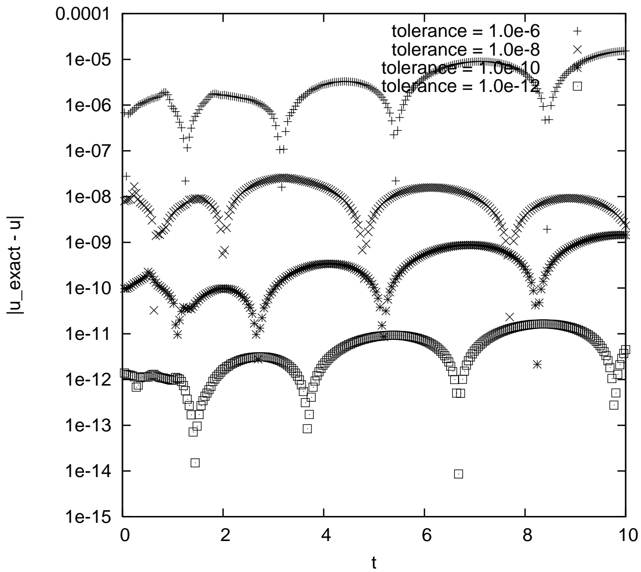
LSODA integration of u''(t) = -u(t)
