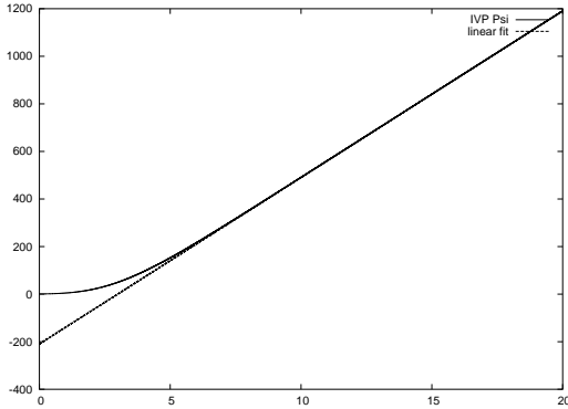
Figure 8: A plot of the solution of the ivp problem along with the linear fit.
