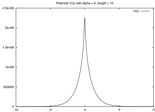
Figure 4: The potential energy function for parameters \alpha = 6 , and x_{max} = 10 . For values of x larger than this, the potential is approximately zero.
